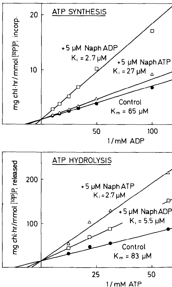
Fig.2. Effects of Naph-ADP and Naph-ATP on ATP formation and ATP hydrolysis. For measurement of ATP hydrolysis different concentrations of ADP were completely phosphorylated to [\gamma\text{-}^{32}\text{P}]\text{ATP} by pre-illumination of a chloroplast suspension for 5 min. Initial rates of ATP hydrolysis were determined by the disappearance of [\gamma\text{-}^{32}\text{P}]\text{ATP} in the following dark period. Additions of Naph-ADP and Naph-ATP, respectively, were made together with turning off the light.
